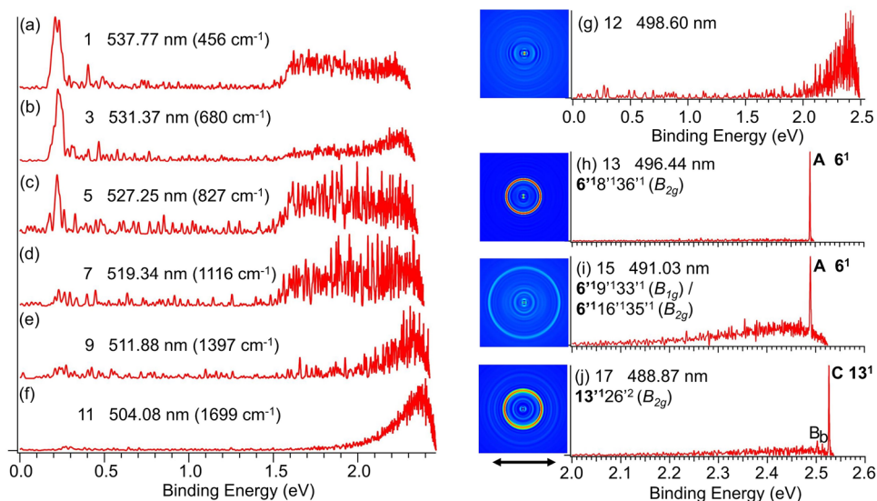
Figure 2. R2PD PE spectra of \text{TCNB}^- for selected below-threshold QBS vibrational levels (a–f) and resonant PE images and spectra for selected above-threshold QBS vibrational levels (g–j). The peak numbers and excitation wavelengths are labeled. The energy shift relative to the 0–0 transition corresponding to each below-threshold vibrational peak is indicated in the parentheses in the left column. In the right column, peaks labeled in boldface with capital letters indicate autodetachment-enhanced vibrational levels in the final neutral \text{TCNB} . The assignments of the above-threshold QBS vibrational levels and their symmetries (in parentheses) are also given. The double arrow below the PE image represents the laser polarization direction.
