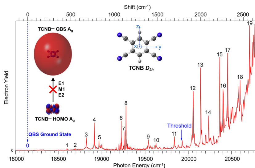
Figure 1. Photodetachment spectrum of TCNB - obtained by monitoring the electron yield as a function of photon energy. Resonant peaks are labeled as 1–19 corresponding to vibrational levels of the QBS. Note the 0–0 transition from the anion ground state (A u ) to the QBS (A g ) is E1, M1, and E2 triply forbidden. It is deduced to be at an excitation energy of 18 139 cm -1 indicated by the dashed arrow and labeled as 0 (see text). The detachment threshold at 19 918 cm -1 is indicated by a short arrow. The molecular structure of TCNB (D 2h ) and the associated coordinates are given in the inset. The HOMO of TCNB - and the QBS (plotted with an isovalue of 0.0004) are also given in the inset. Note the \sigma -like symmetry and the diffuseness of the QBS orbital.
