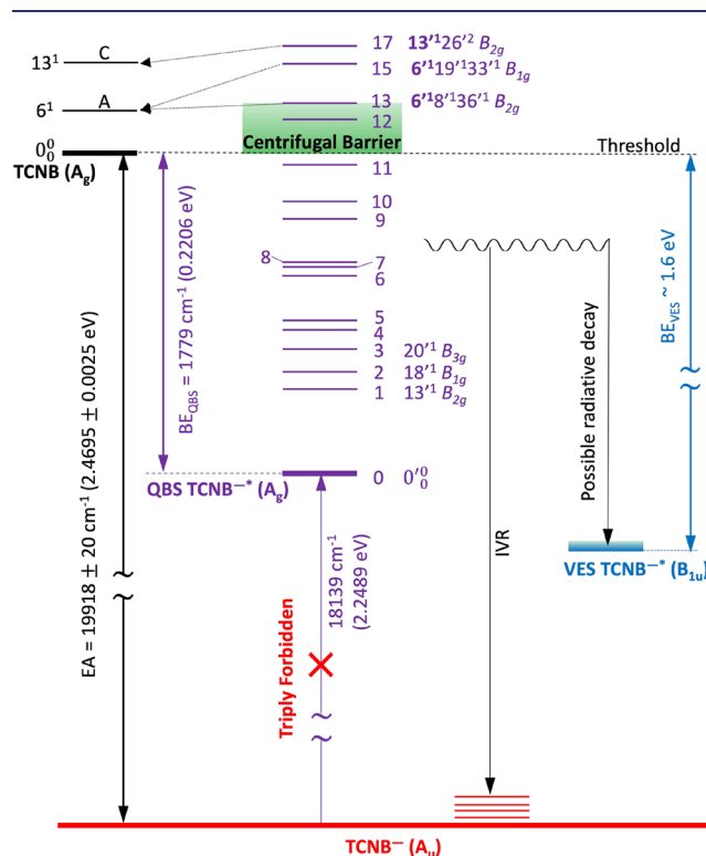
Figure 3. A schematic energy level diagram showing the autodetachment from the QBS vibrational levels of TCNB^- to the neutral vibrational manifold of TCNB (left). The possible radiative decay to the VES and relaxation to the vibrational manifold of the anion ground state via IVR (right), as well as the centrifugal barrier in the near above-threshold region (middle), are also shown. See Figure S5 for a more complete diagram.
